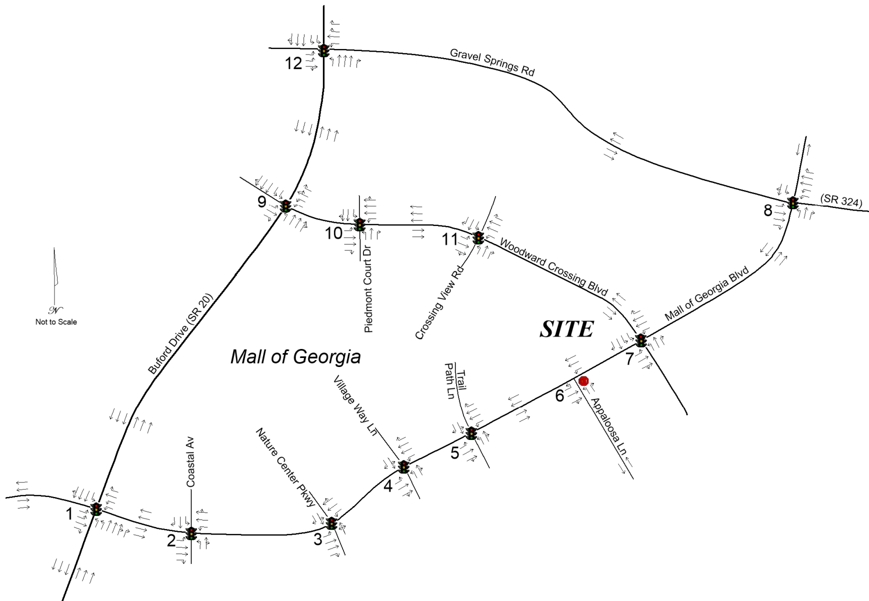
Figure 6 – Existing Lane Configuration and Traffic Control
